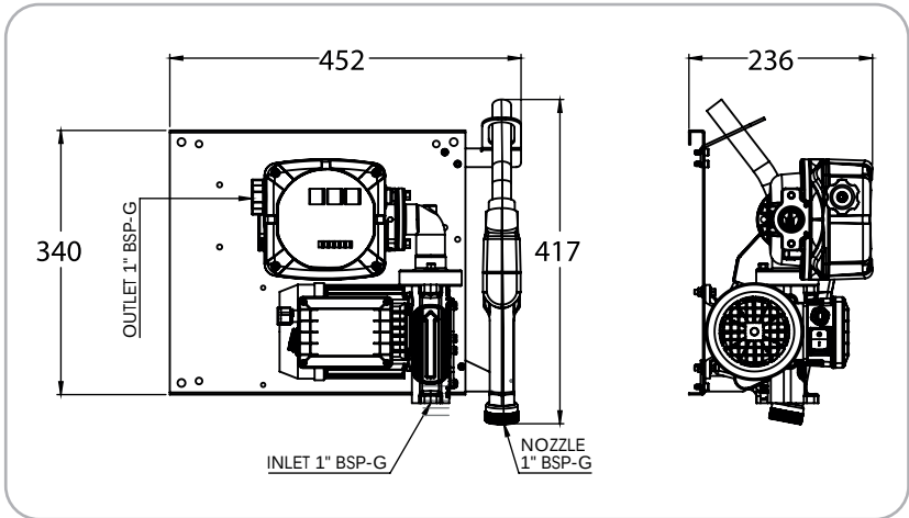
Ingombri - Overall Dimensions (mm)
