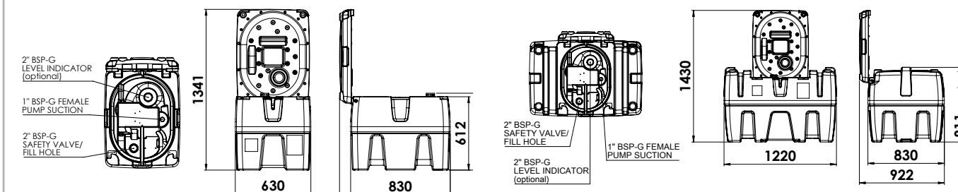
Ingombri - Overall Dimensions (mm)
