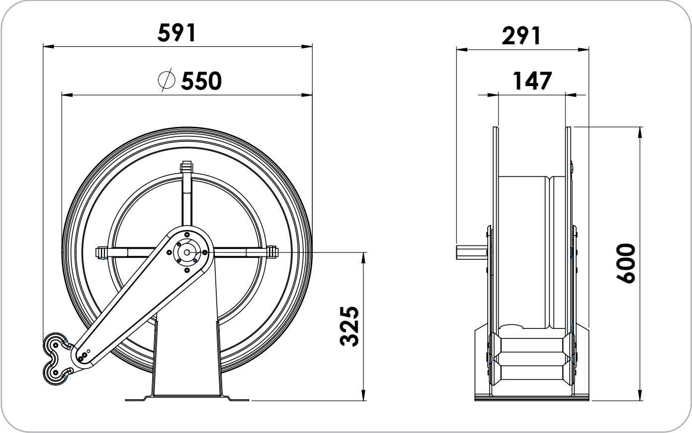
Ingombri - Overall Dimensions (mm)
