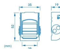
ref. o TCS25 t.c.s. buckle, 25 mm t.c.s. buckle, 25 mm
