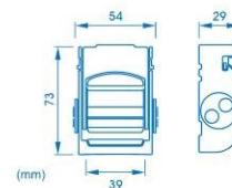
ref. o TCS35 t.c.s. buckle, 35 mm t.c.s. buckle, 35 mm
