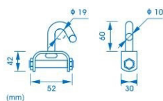
ref.ª G5000PC50 gancho porta carro, 50 mm tire holder hook, 50 mm
