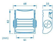
ref. o TCS50 t.c.s. buckle, 50 mm t.c.s. buckle, 50 mm
