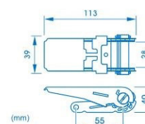
ref.ª T1T25 tensor standard, 800 kg standard ratchet, 800 kg
