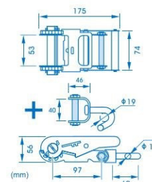
ref.ª T5T50PCC porta carro completo, 5000 kg complete tire holder, 5000 kg
