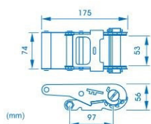
ref.ª T5T50PC porta carro, 5000 kg tire holder, 5000 kg
