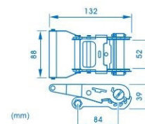
ref.ª T2T50 pega curta, 2000 kg short handle, 2000 kg
