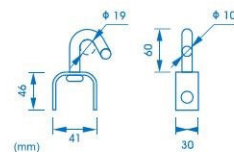
ref.ª G5000PC40 gancho porta carro, 40 mm tire holder hook, 40 mm
